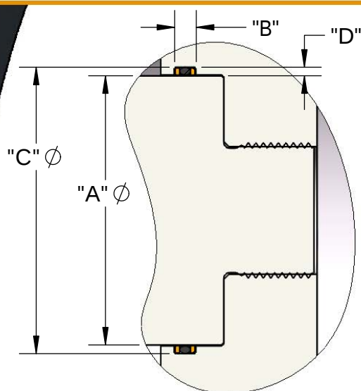
Reference Groove Dimensions for O-rings with "G" back-up rings
